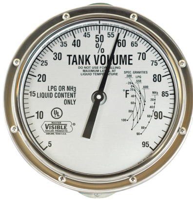
130035 - Master Dial Mounts to 2 Tabbed Heads LP or NH3 8" Master
