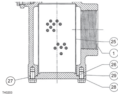
Figure 3. Type C402 Strainer Parts
