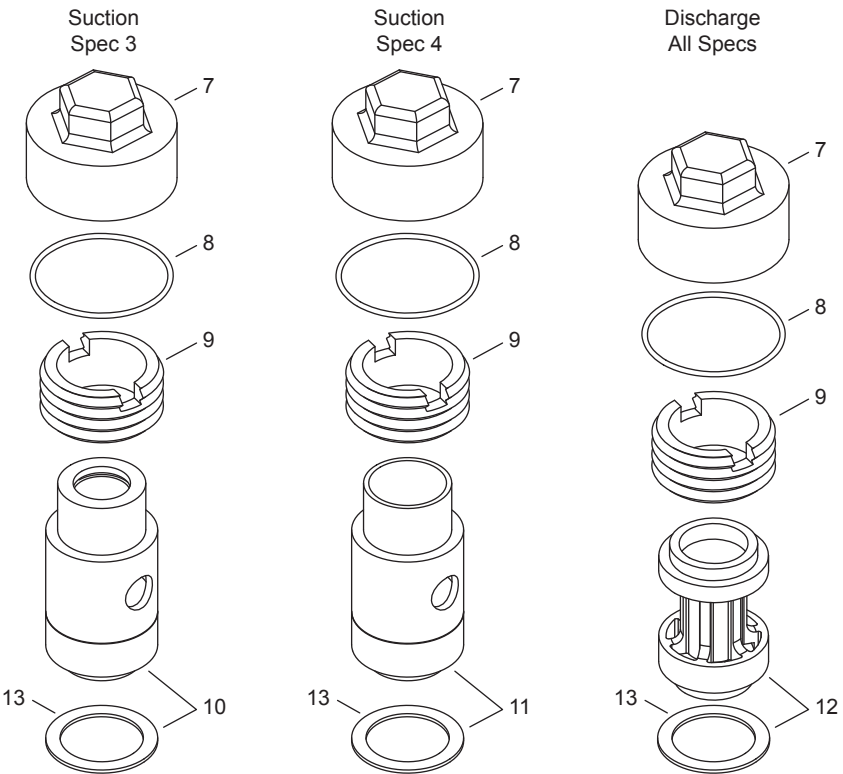
Valve Holddown Assemblies
