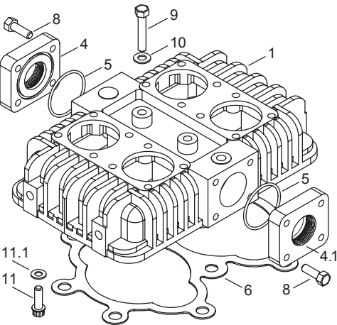
690 Head Assembly
