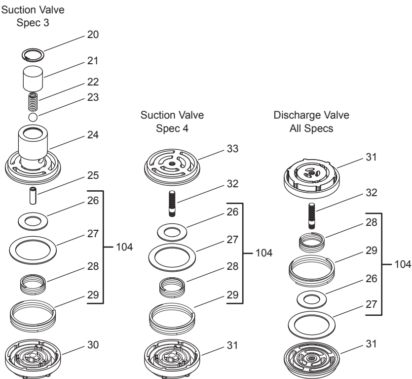
Valve Assemblies
