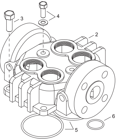
F291 Head Assembly
