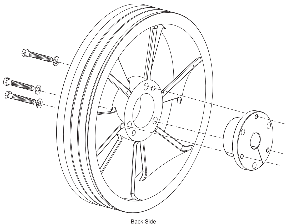
Flywheel Assembly Bill of Materials
