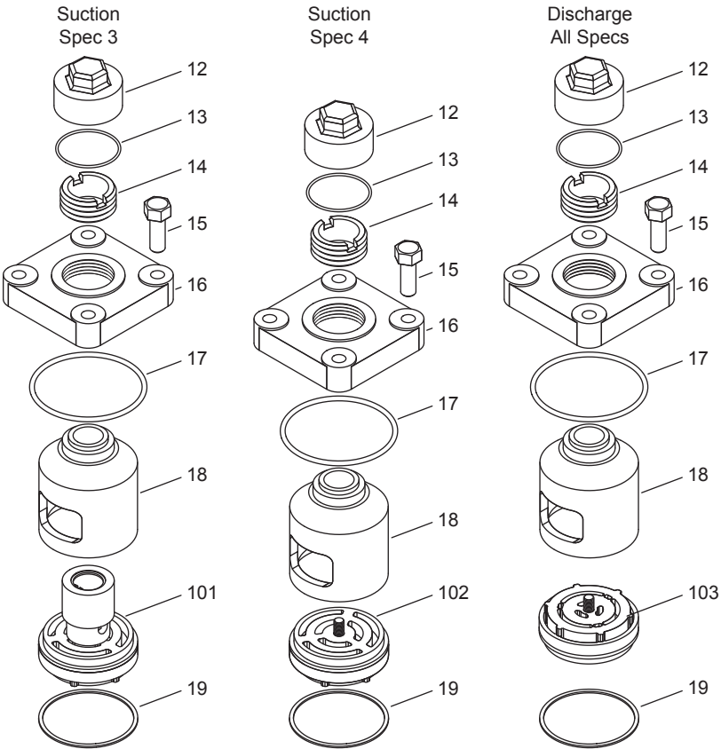
Valve Holddown Assemblies
