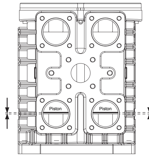
Piston bottom dead center
