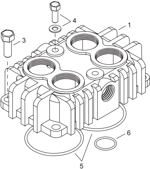
291 Head Assembly
