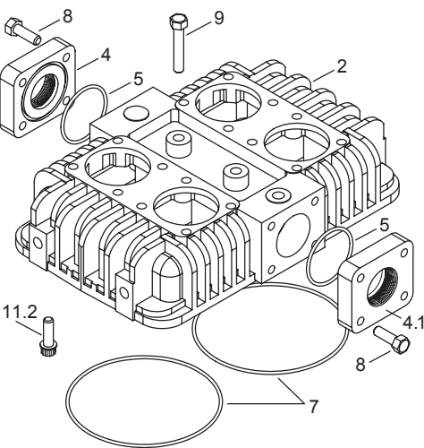
691 Head Assembly
