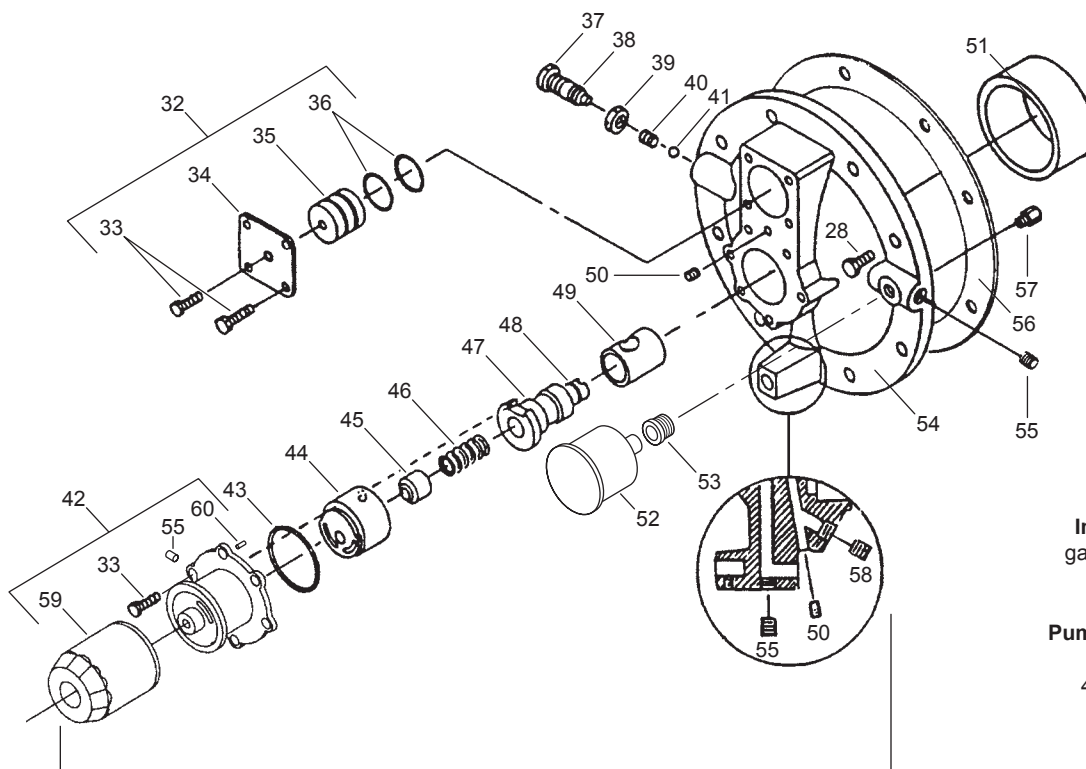
Inside of Bearing Carrier
