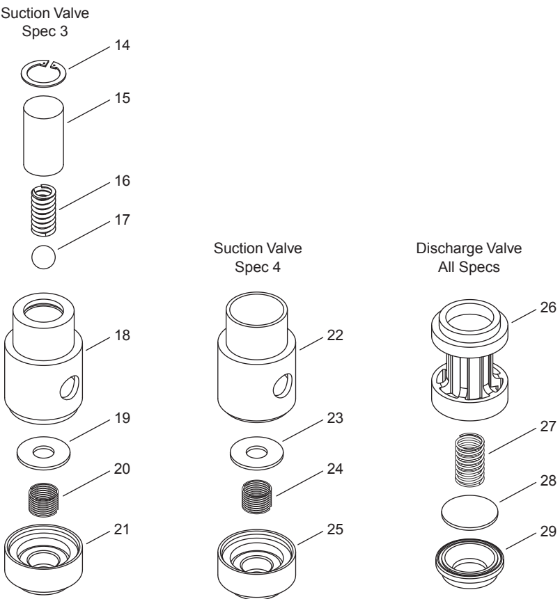
Valve Assemblies Details
