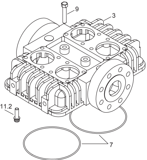
F691 Head Assembly
