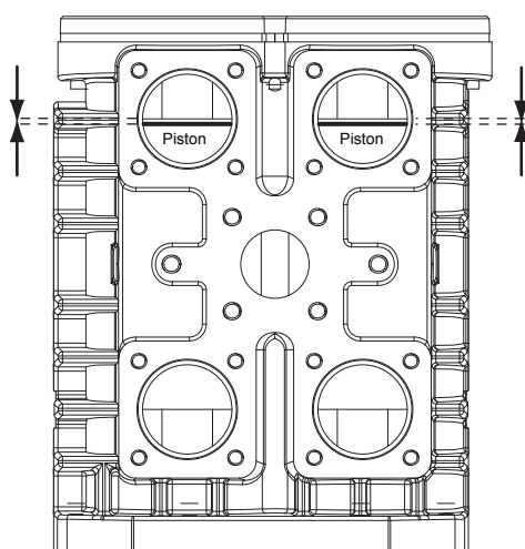
Piston top dead center
