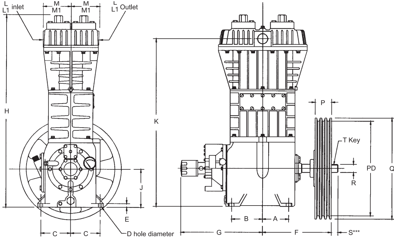
Outline Dimensions—Inches (Centimeters)
