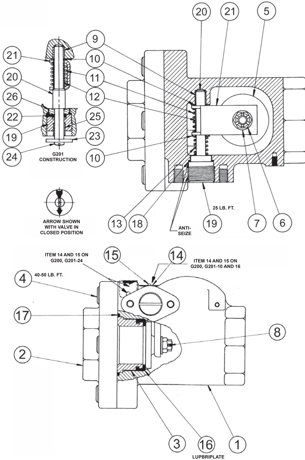
Figure 1. G200 Back Check Valve
